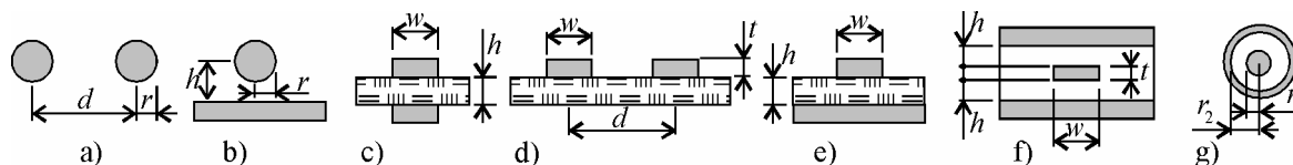
Obr.4.8: Impedance.
