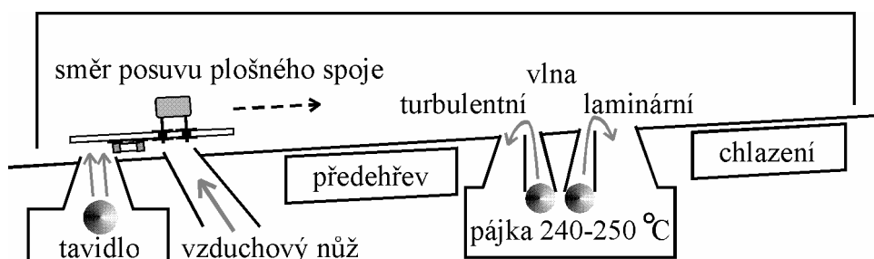
Obr.3.8: Princip vlny.
