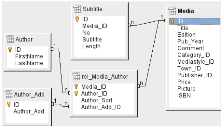
Figure 35: Example 1:n relationship; n:m relationship
