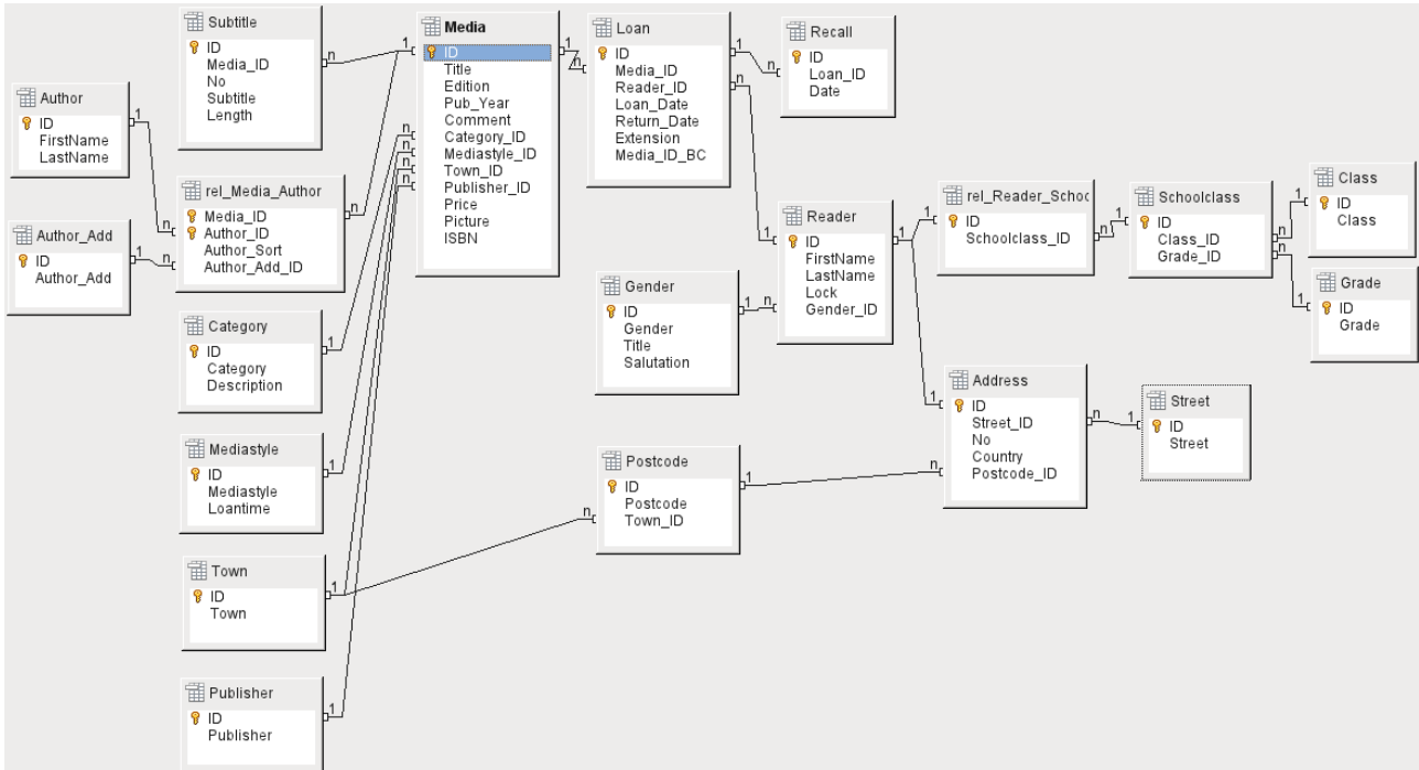
Figure 34: Relationship diagram for the example database media_without_macros
