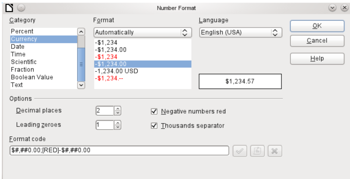
Figure 85: Formatting numbers
