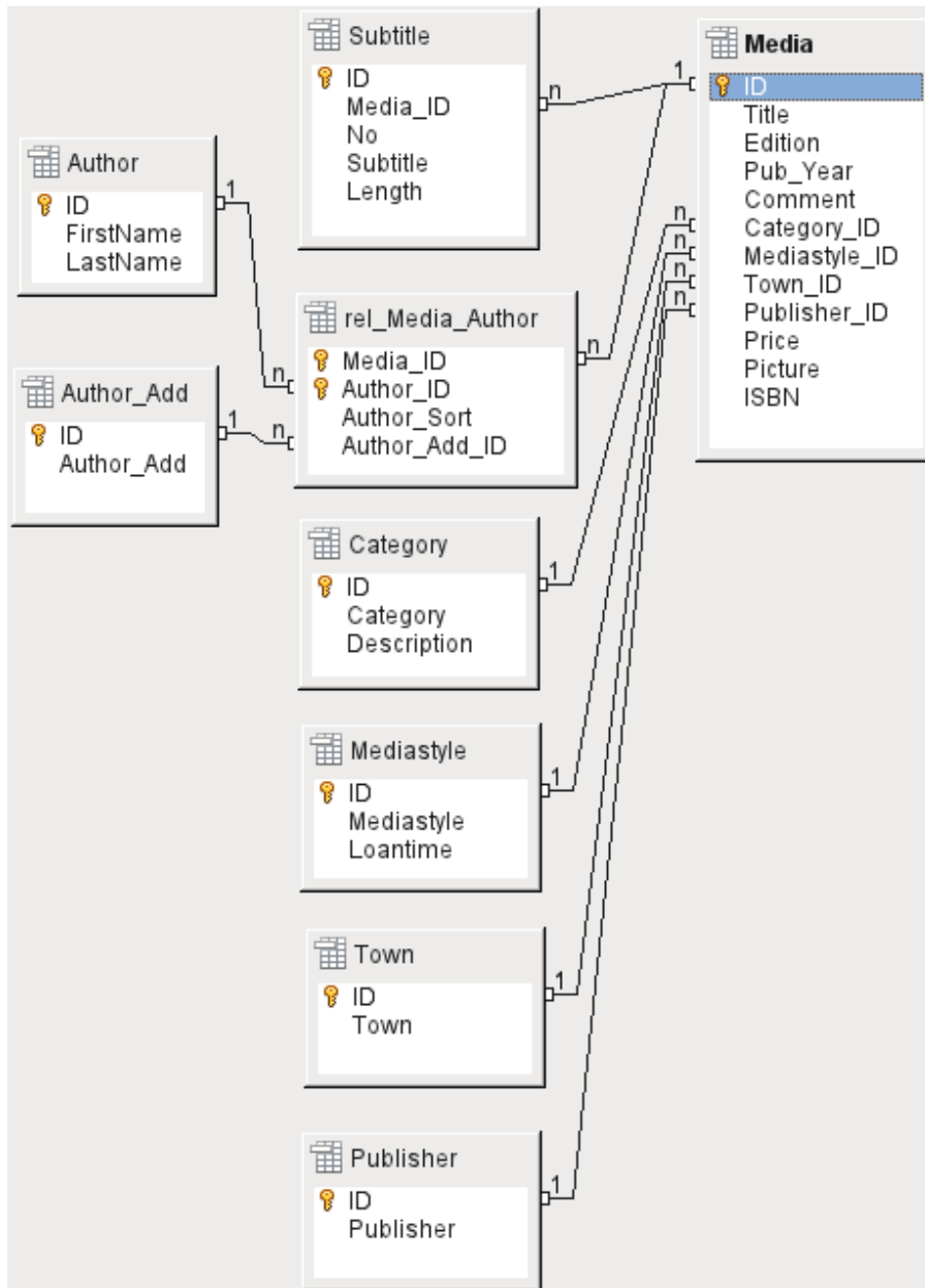
Figure 37: Media addition
