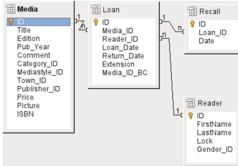
Figure 38: Loan
